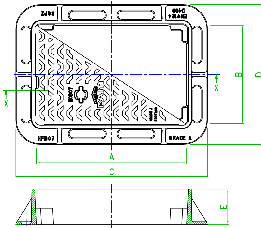
Section X-X (Frame only)
