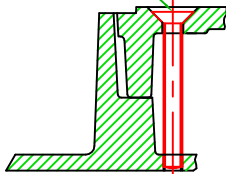
TYPICAL SCRAP SECTION SHOWING OPTIONAL LOCKING OF COVER TO FRAME HB02&3 ONLY.
