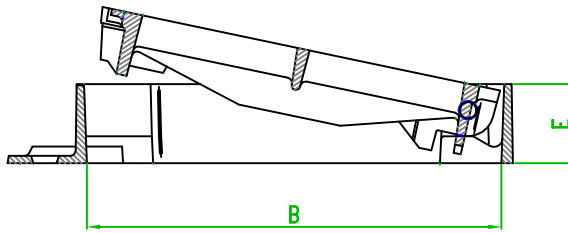
SECTION X-X
