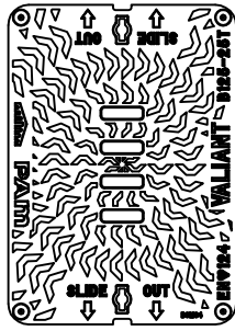
Vented cover detail.
