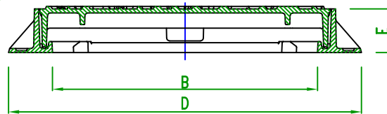
Section Y-Y
