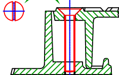
TYPICAL SCRAP SECTION SHOWING OPTIONAL BOLTING DOWN OF COVER TO FRAME
