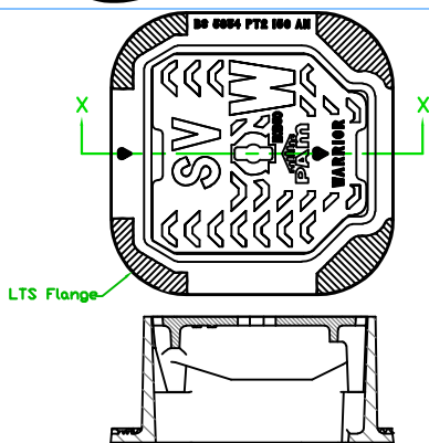
SECTION X-X PLAN & SECTION FOR FSWA15CK
